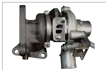
Fig 3: EREV turbocharger
