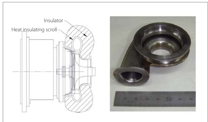
Fig 6: Turbocharger improvement The turbine scroll was made thinner and wrapped with heat insulator in an effort to increase turbine power.
