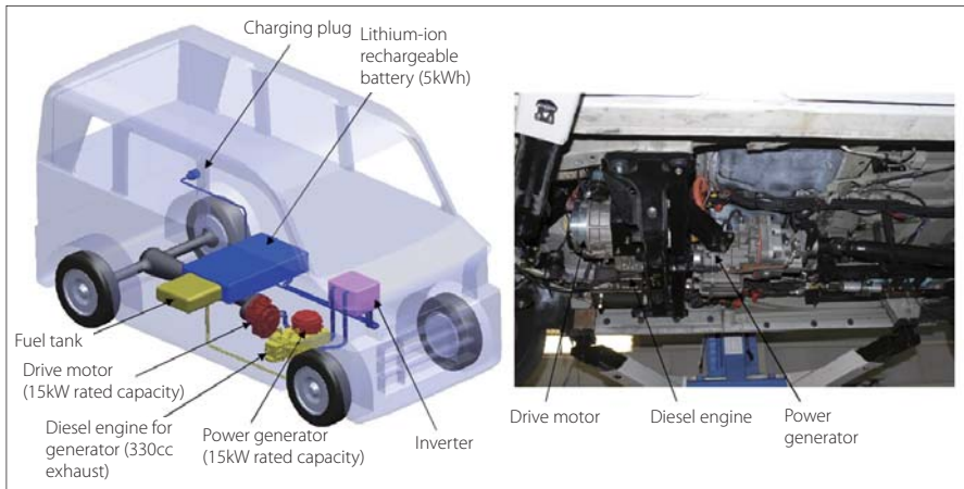
Fig 2: Components of an EV micro diesel power generator
