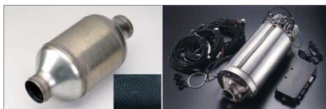
Fig 1: ACR EXCAT and ACR DPF
