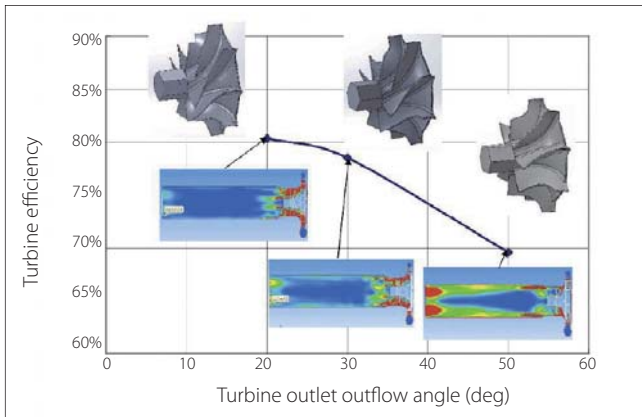
Fig 5: Evaluation of turbocharger vane geometry using simulations Results show that reducing the turbine rotor vane outflow angle reduces the generation of heat around the rotor vane outlet and improves performance. The turbine angles are 50, 30, and 20 degrees from right. Contour diagrams of friction heat are shown below.
