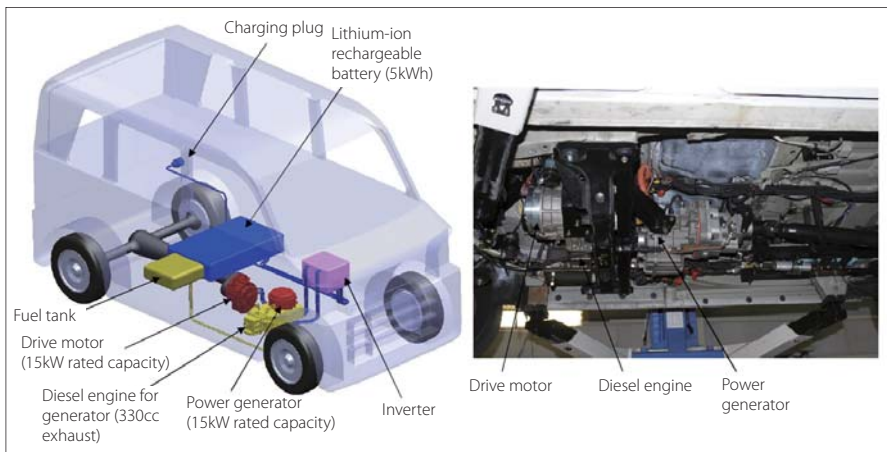
Fig 2: Components of an EV micro diesel power generator
