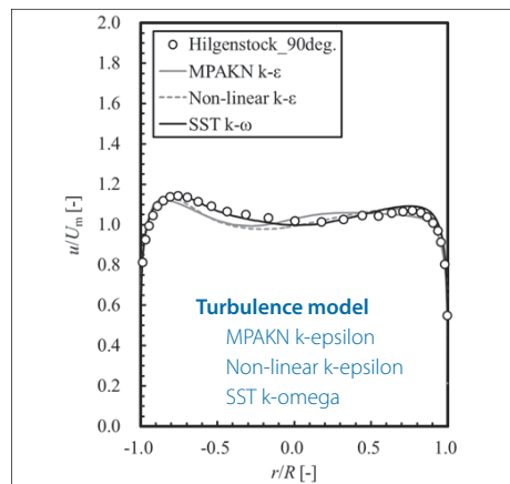
Fig 2: Comparison between analysis and experiment values undertaken by Hilgenstock et al. *2 Results using SST k-\omega model were in closest agreement with experiment values.
