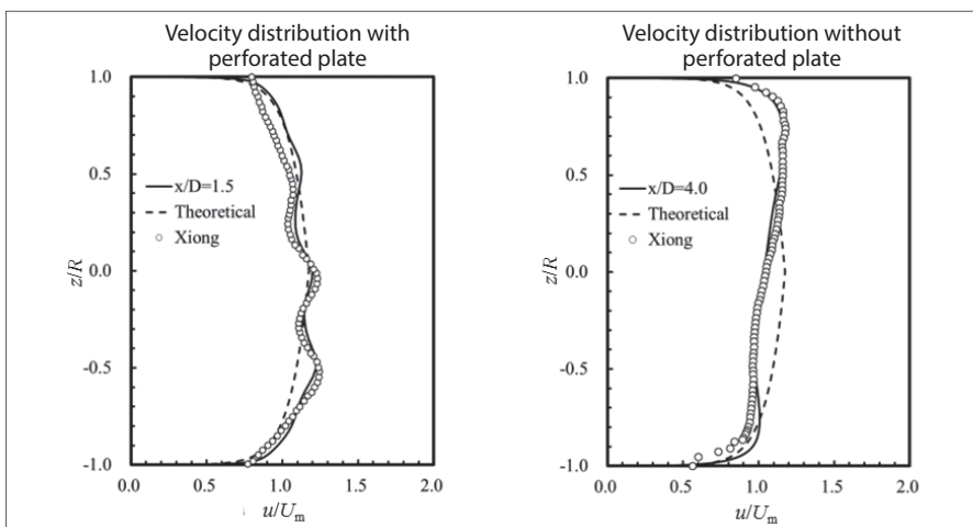
Fig 5: Velocity distribution Analysis results were in close agreement with experiment when SST k-\omega model was used.
