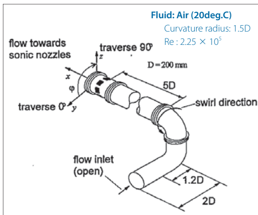
Fig 1: Comparison between velocity distribution near flow inlet and outlet (experiment conditions tested by Hilgenstock et al. *2 )
