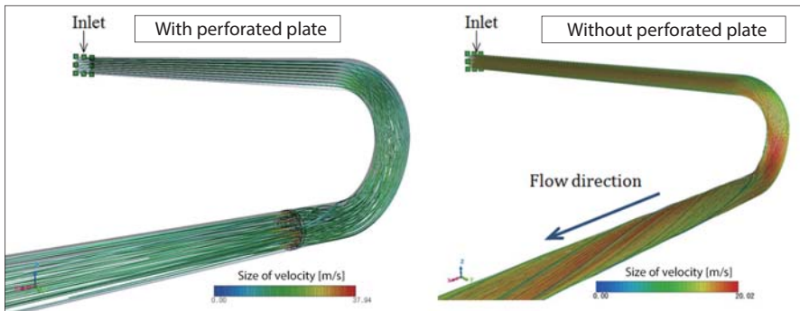
Fig 4: Streamlines shown in the analysis results calculated using SST k-\omega model. Swirling flow occurs without perforated plate.
