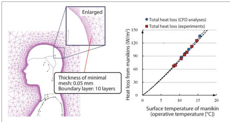
Fig 1: Comparison between fluid analysis and experiment results on a thermal manikin showing thermal conductivity
