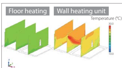
Fig 2: Difference between temperature distribution for thermal manikin depending on types of heating
