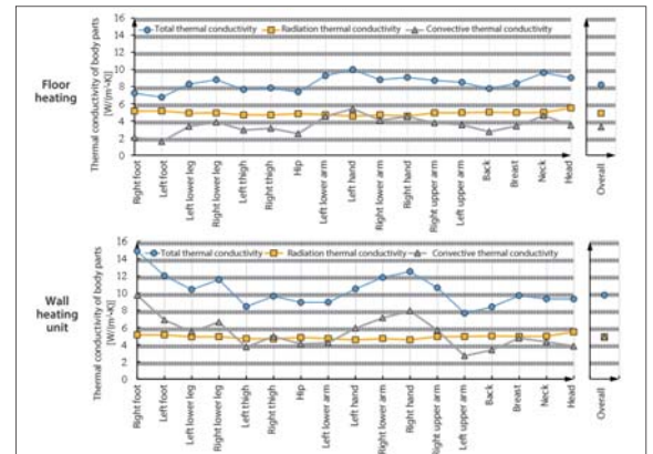
Fig 3: Analysis results of human thermal conductivity between two types of heating
