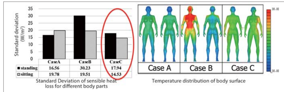
Fig 5: Analysis results of human thermal conductivity when using different types of heating
